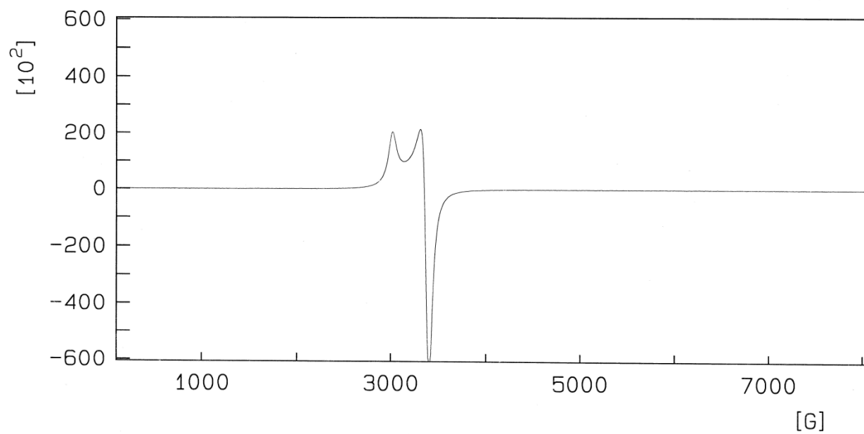
The ESR spectrum of copper complex (5)
