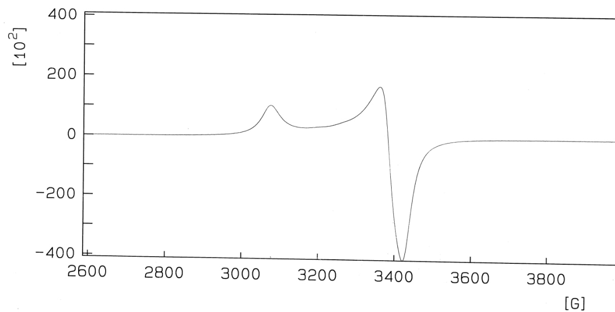
The ESR spectrum of copper complex (4)
