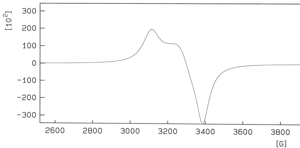
The ESR spectrum of copper complex (3)
