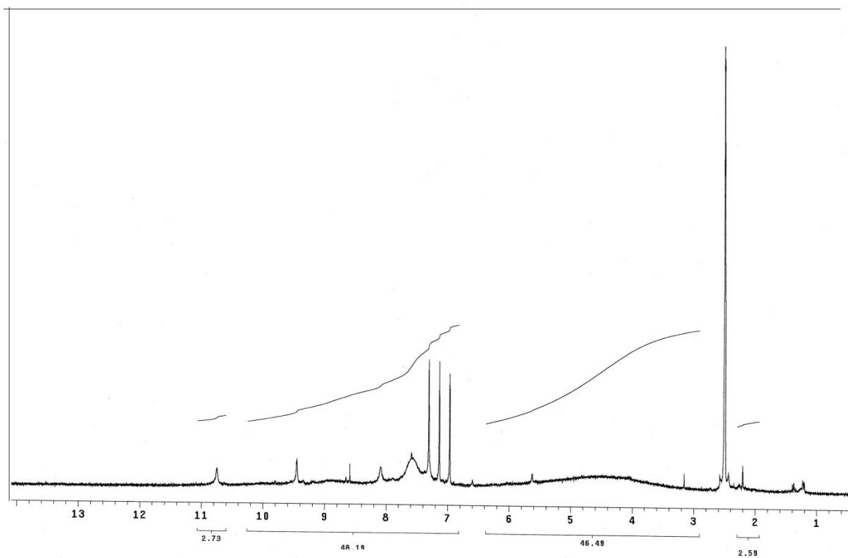
The ^1\text{H} NMR spectrum of ligand ( \text{H}_2\text{L} )
