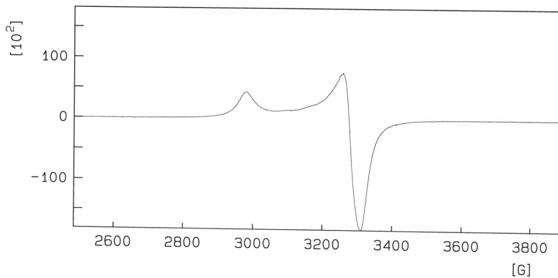
The ESR spectrum of copper complex (2)
