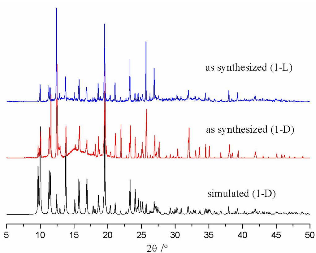
Figure S5. PXRD patterns of 1-D and 1-L
