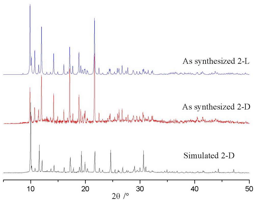
Figure S6. PXRD patterns of 2-D and 2-L
