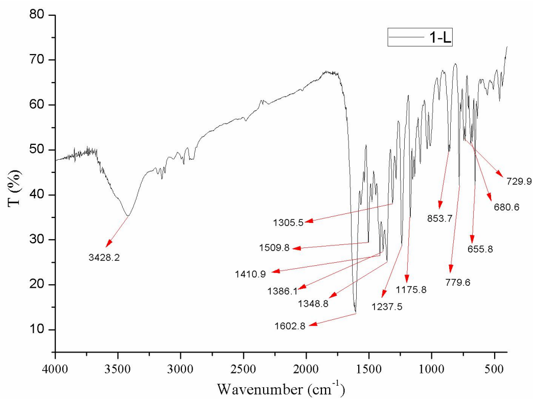
Figure S2. The IR spectra of 1-L
