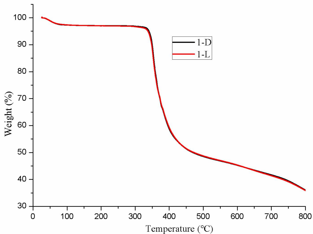
Figure S7. TGA curves of 1-D and 1-L
